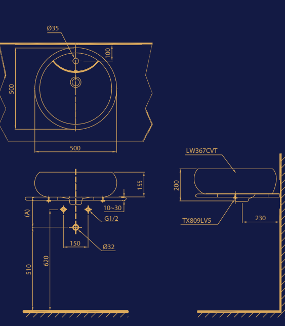
Product dimension: L500 x W500 x H200 (mm)
