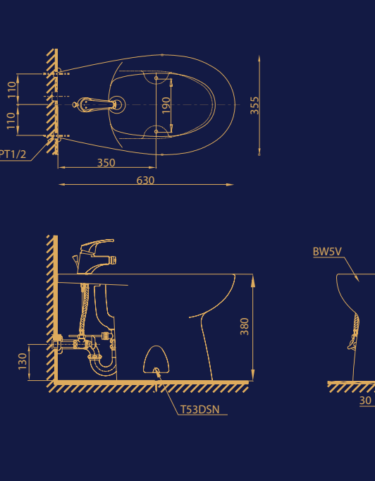
Product dimension: L630 x W355 x H380 (mm)
