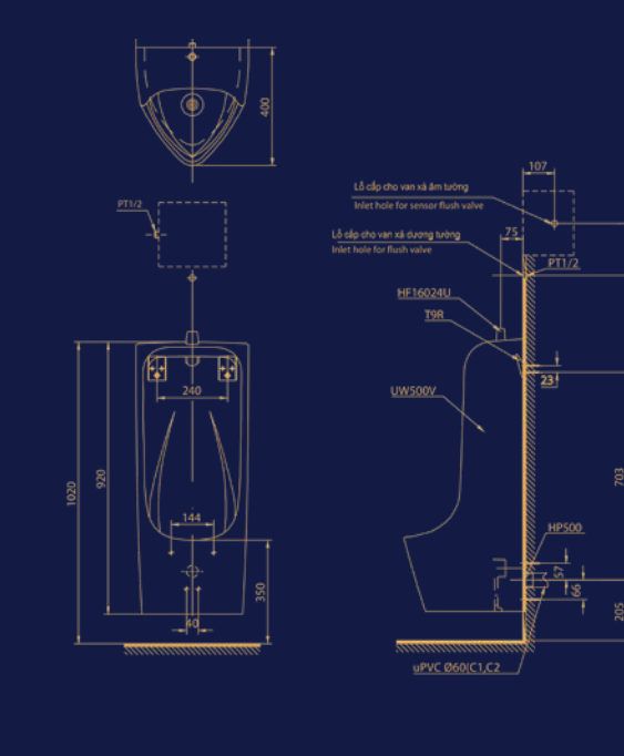
Product dimension: L400 x W380 x H920 (mm)
