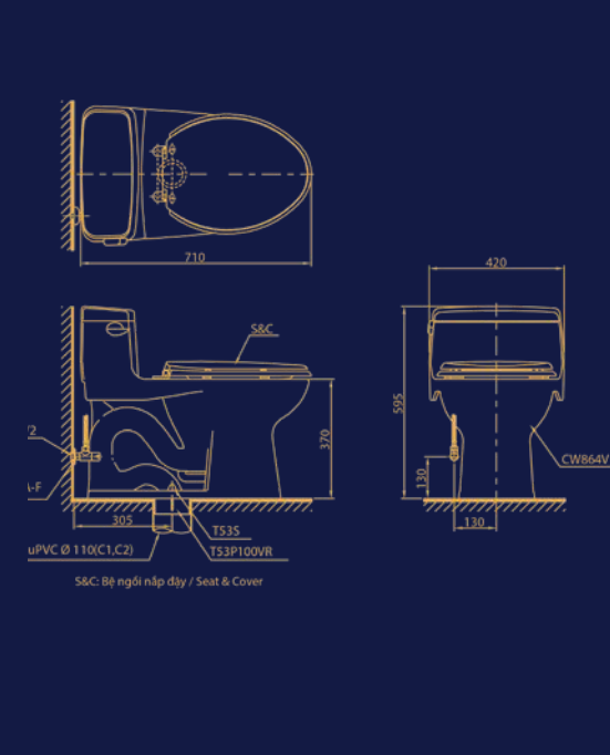
Product dimension: L710 x W420 x H595 (mm)
