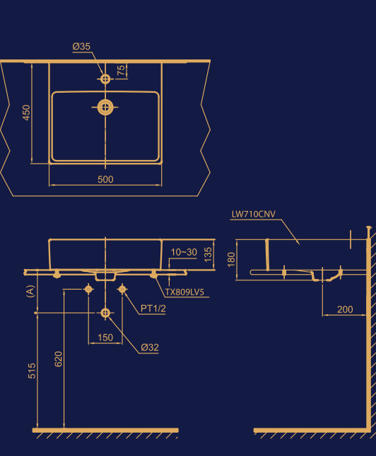
Product dimension: L450 x W500x H180 (mm)
