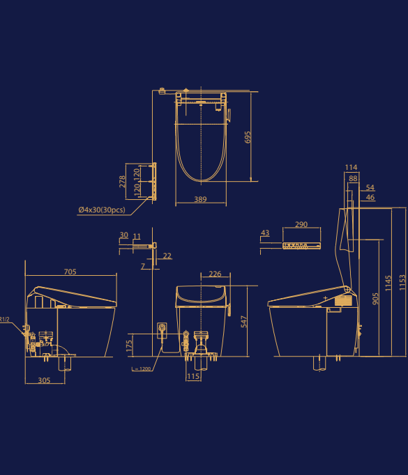
Product dimension: L695 x W389x H547 (mm)
