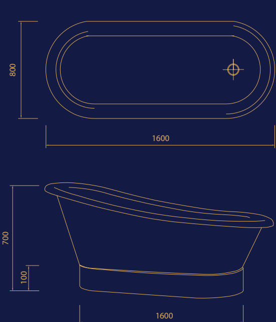
Product dimension: L1600 x W800 x H700 (mm)
